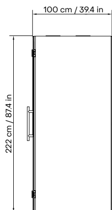
RIGHT VIEW
