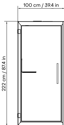
FRONT VIEW
